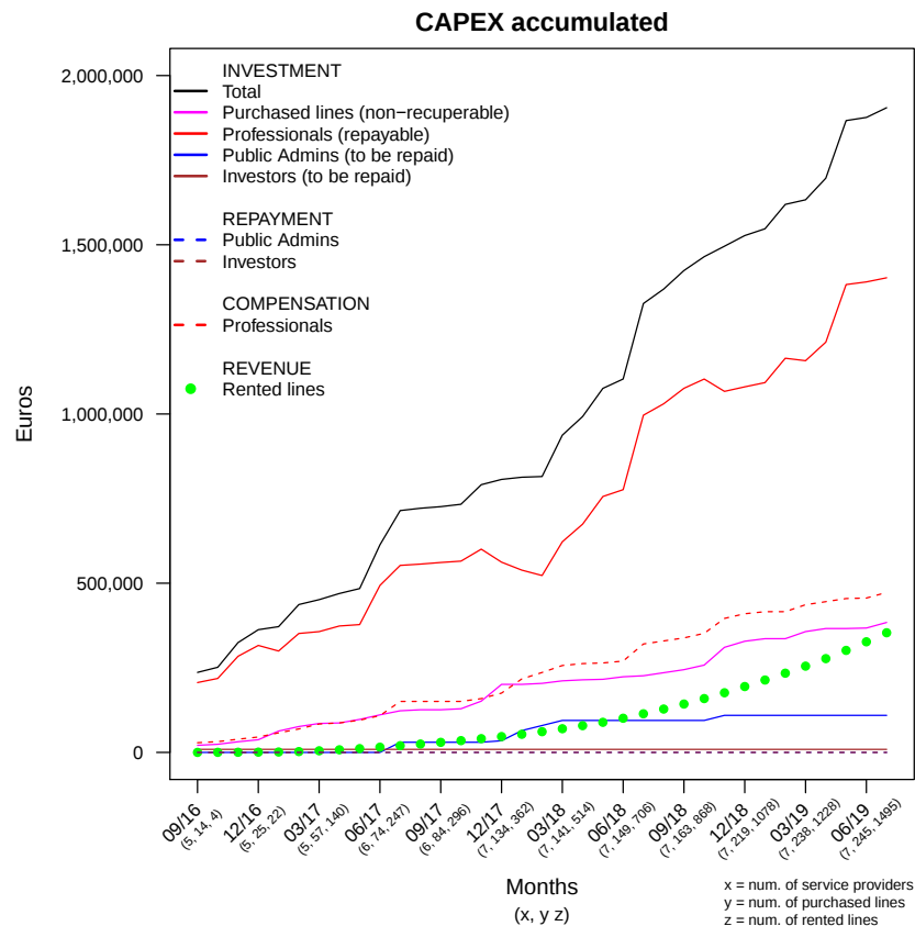
Figure 3.2: Accumulated investment in OF in Xarxa de fibra òptica de la Garrotxa (XAFOGAR) (Source: Guifi.net foundation).
