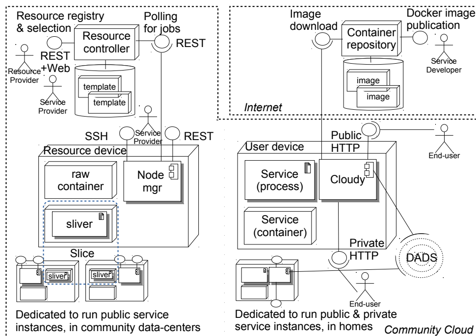
Figure 7.3: Structure and components of a CC deployment.
