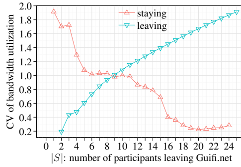
Figure 5.10: coefficient of variation (CV) of the participants' bandwidth usage, u_p , in each staying \bar{S} and leaving S sets. The lower the CV is, the more balanced the sets are.
