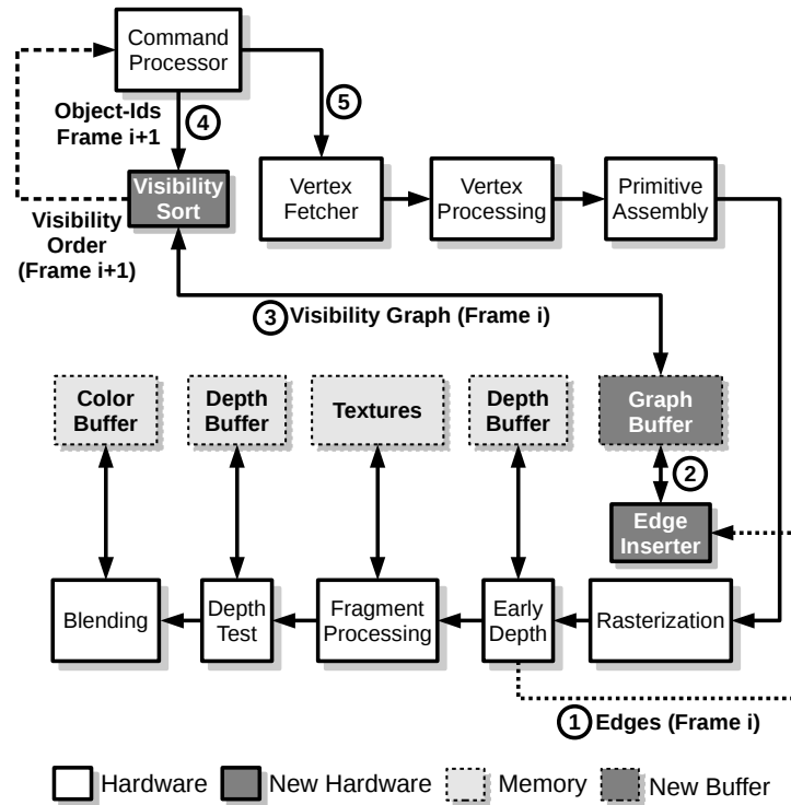
Figure A.2: Graphics pipeline including VRO.
