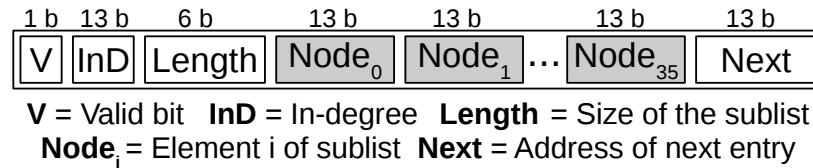
Figure 4.11: Detail of an entry of the Graph Buffer. Each entry is 512 bits (including 11 bits of padding).
