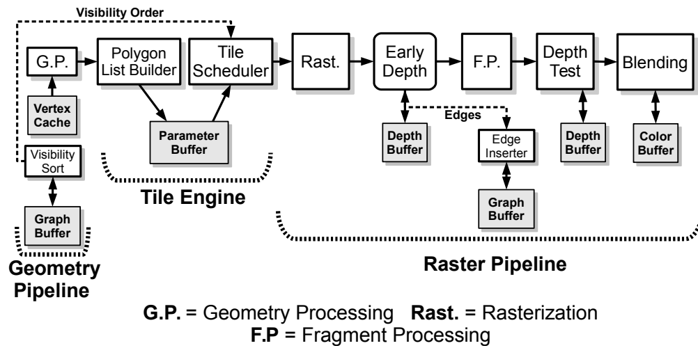
Figure 4.4: Graphics pipeline including VRO.
