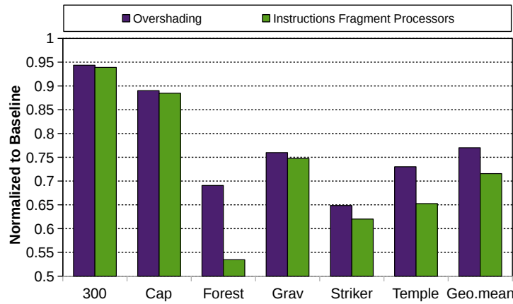
Figure A.7: Overshading and Instructions Executed in the Fragment Processors with IMR-VRO normalized to those of the baseline IMR GPU.
