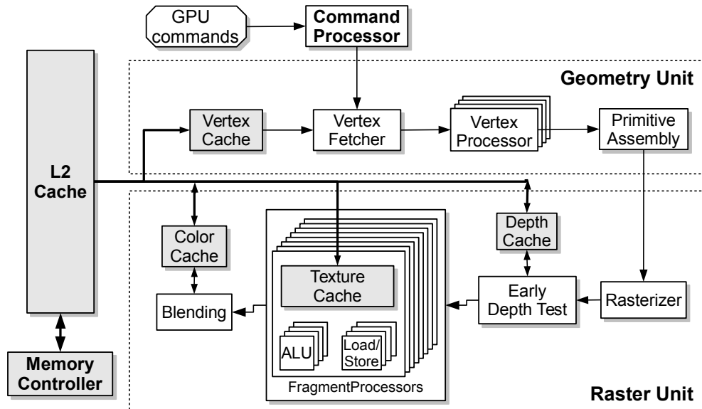
Figure 2.14: Microarchitecture of an IMR GPU.
