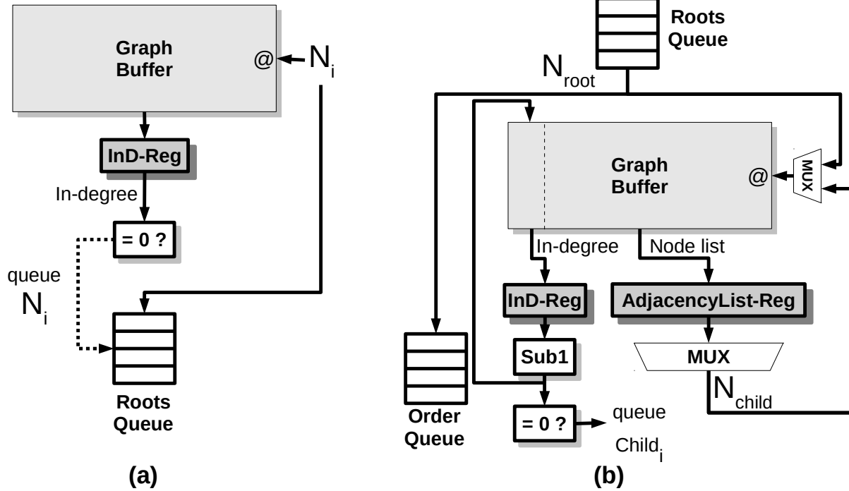
Figure 4.15: Visibility Sort Hardware. (a) Initial search (b) Iterative procedure
