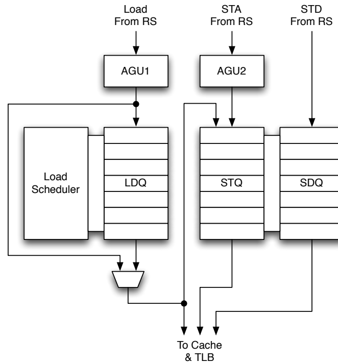
Figure 2.1: Simplified Schema of the P6 Memory Unit.
