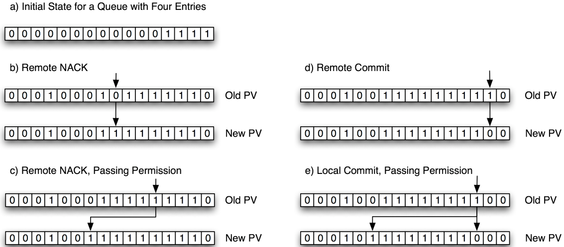
Figure 5.13: Updates of the Permission Vector (PV).
