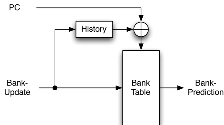
Figure 3.6: Gshare Bank Predictor.
