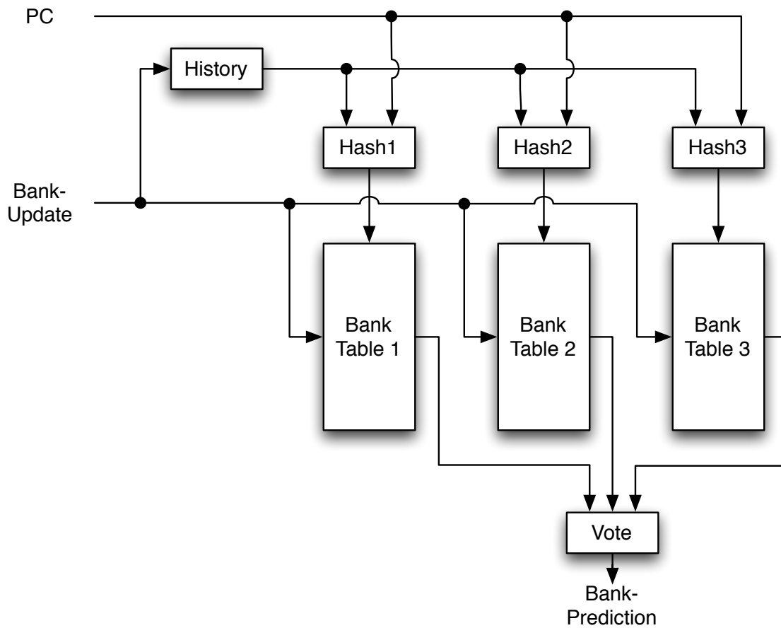
Figure 3.17: Gskew Predictor.
