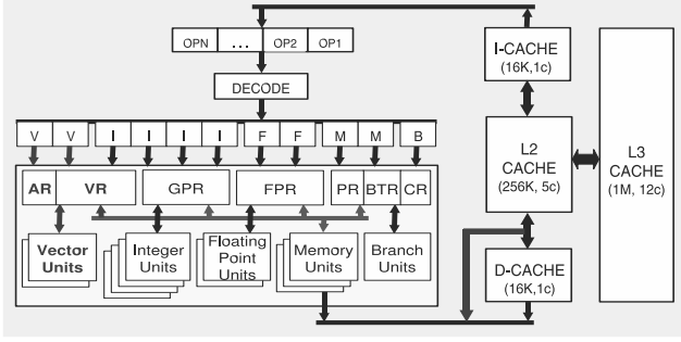
Figure 2. Vector- \mu SIMD-VLIW architecture
