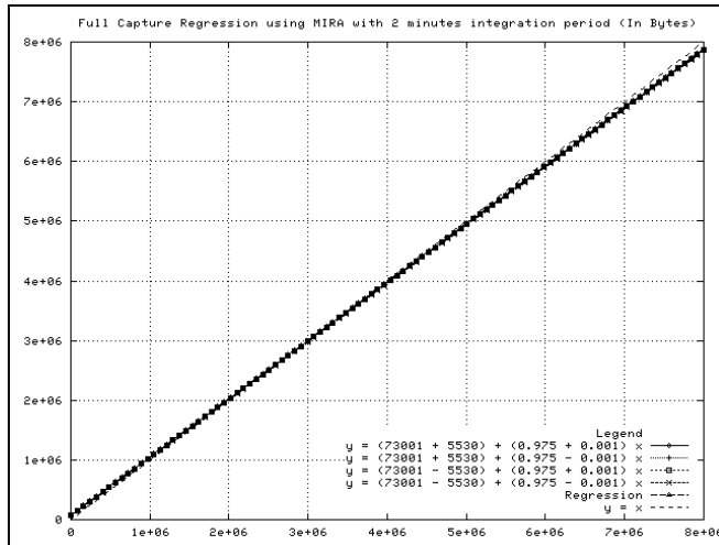
Figure4. SLR Straight lines for Input traffic in bytes, with two minutes integration period.
