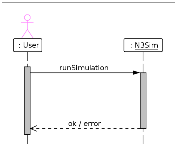
Figure 4.2. sequence diagram for the use case "Run Simulation".
