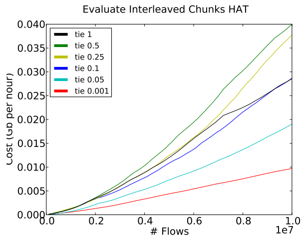
Fig. 3: Impact of the Tie Threshold parameter
