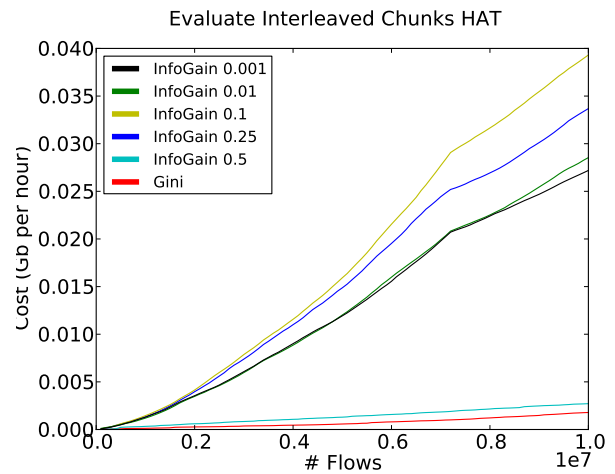
Fig. 4: Impact of the Split Criteria parameter
