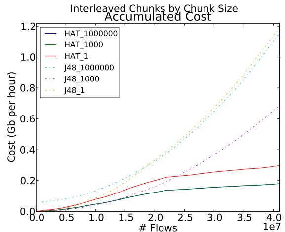
Fig. 10: Accumulated cost by chunk size
