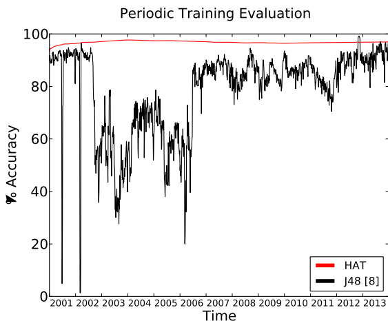
Fig. 11: Interleaved Chunk comparison with [8] configuration
