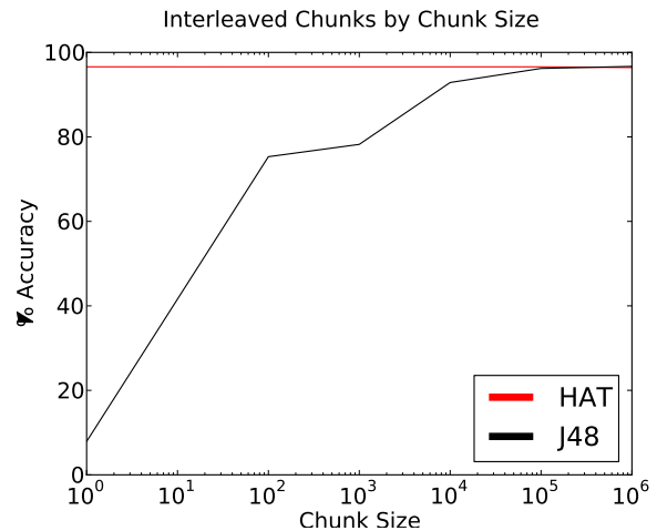
Fig. 8: Accuracy by chunk size
