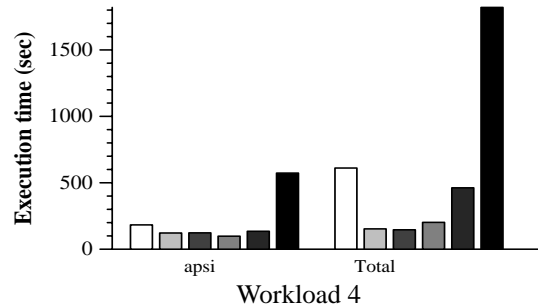
Figure 6: Per application (avg) and total execution time of the parallel workloads.
