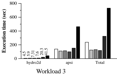
Figure 6: Per application (avg) and total execution time of the parallel workloads.
