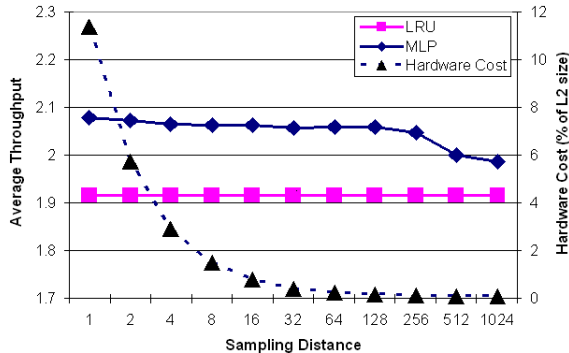
Fig. 10. Average IPC and hardware cost depending on the sampling distance in a two-core CMP
