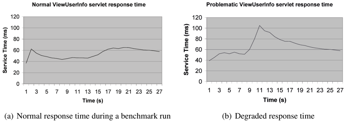
Figure 3.10 Observed response time for a servlet of the RUBiS Benchmark
