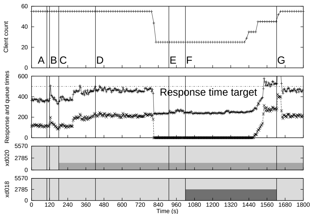
Figure 5.33 Response time for StockTrace and job placement on nodes.
