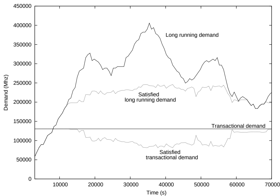
Figure 5.25 Heterogenous workload: CPU power allocated to each workload and CPU demands to achieve maximum utility
