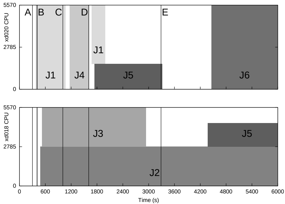
Figure 5.32 Node utilization by long running jobs.
