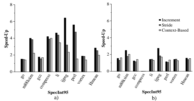
Figure 5: Speed-ups for the different value predictors and for the a) loop-iteration and b) subroutine-continuation spawning schemes.
