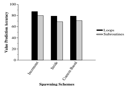
Figure 6: Value prediction accuracy for the different spawning schemes.
